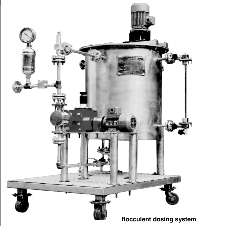
BOILER FEED WATER TREATMENT CHEMICAL DOSING SYSTEM
