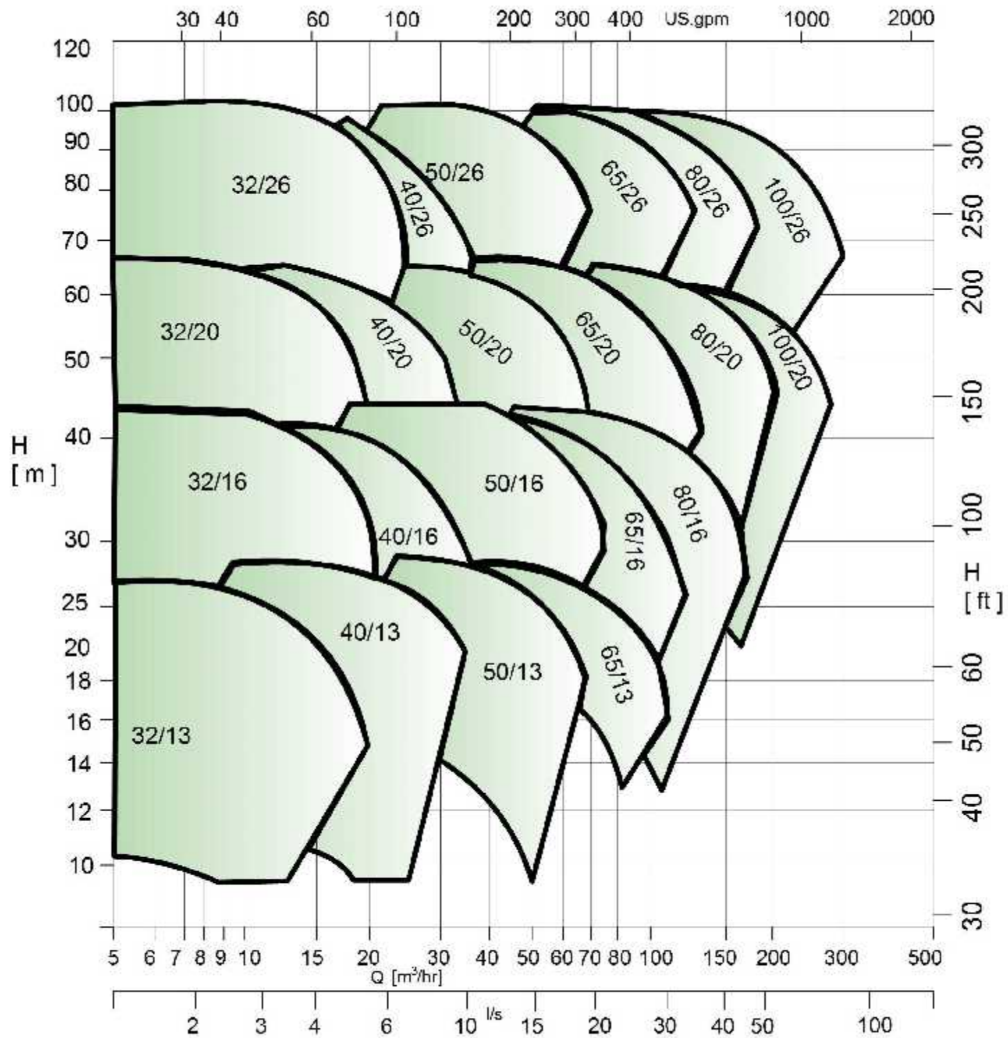
IPKB 2900 RPM
